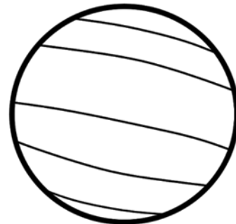
Neptune
